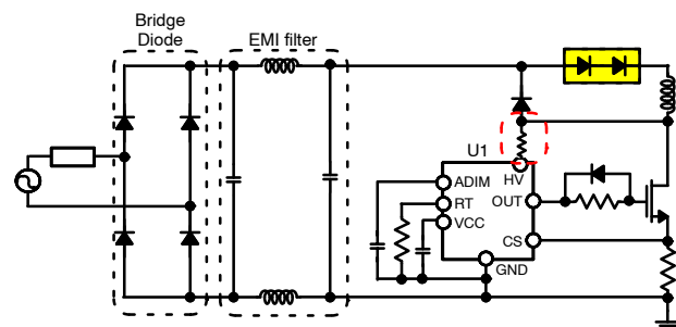
Figure 6. High-Voltage Application
